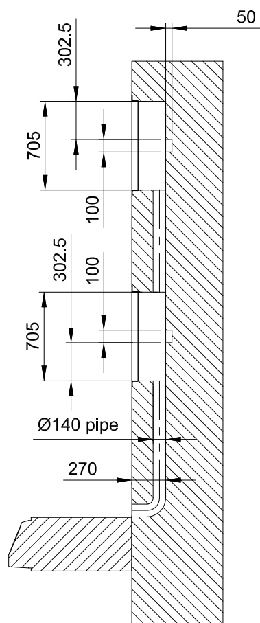
Section B-B
